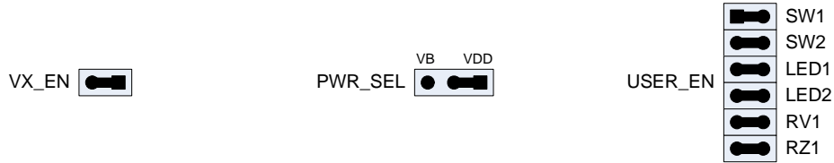
Figure 5. DEMO9S08QG8 Jumper Settings
